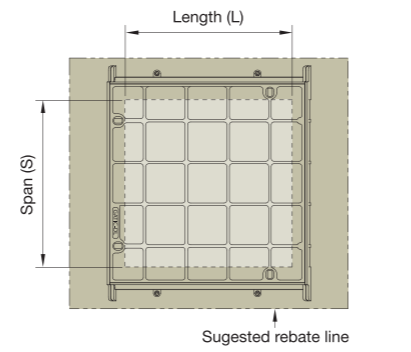
Plan of recessed single cover
