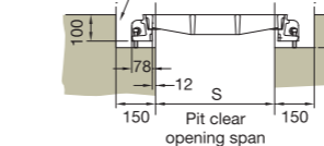
Section through drainage trench
