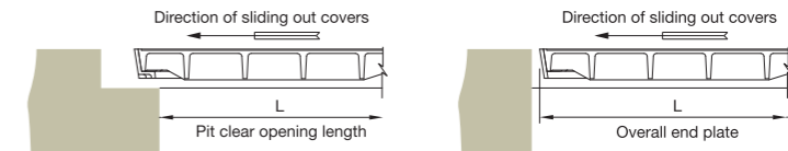
End terminations
