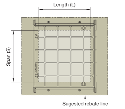
Plan of recessed single cover
